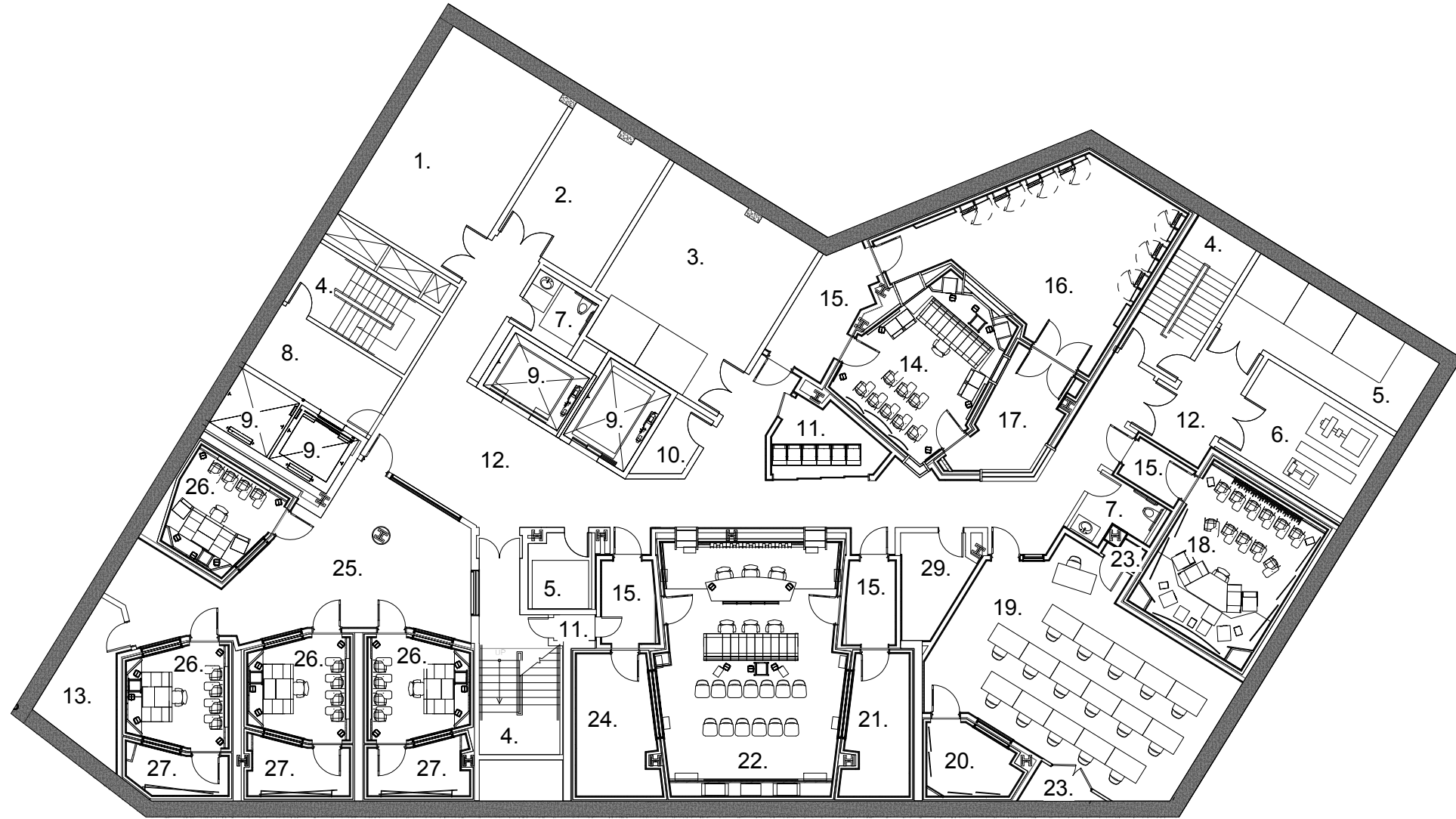
LEVEL B2 - FLOOR PLAN
