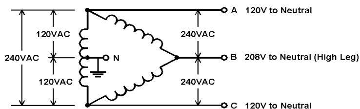
Fig 8 -High Leg Delta
