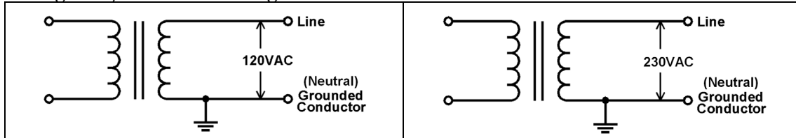
Fig 2 – Single Phase systems
