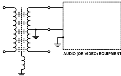
Figure 19c – Isolation Transformer showing inductance of earthing path
