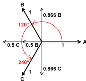
Fig 7a Neutral current at 50/60 Hz
