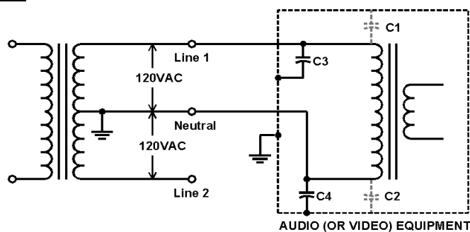
Fig 15 –A Conventional Un-Balanced Power System
