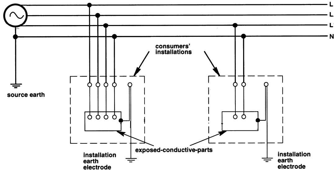
Fig A-4 – TT system
