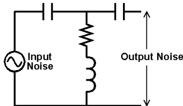
Figure 19d- Equivalent circuit
