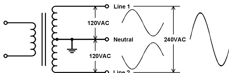
Figure 1 – Single Phase 120V/240V Power System ("split single-phase")
