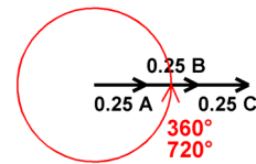
Fig 7b Neutral current for 25% third harmonic
