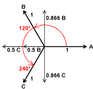
Figure 4a – 3-Phase Voltages
