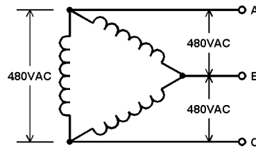
Fig 6 – 480V Delta
