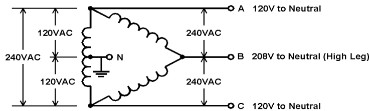
Fig A-6 -High Leg Delta
