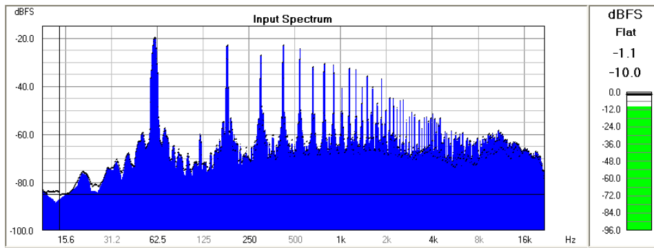
Fig 17 – Typical noise spectra on a equipment ground
