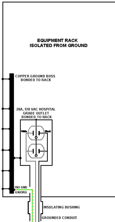
Fig 14b – Equipment Rack Wiring
