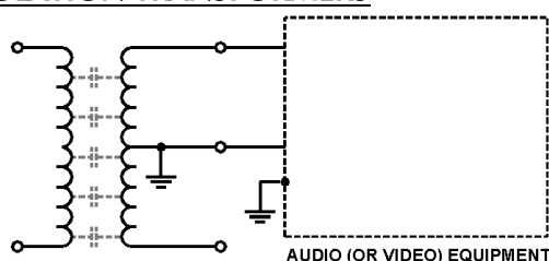
Figure 19a – An Ordinary Transformer
