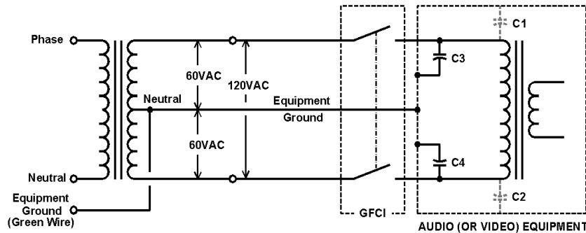
Fig 16 –A Balanced Power System per NEC 647 (2002)
