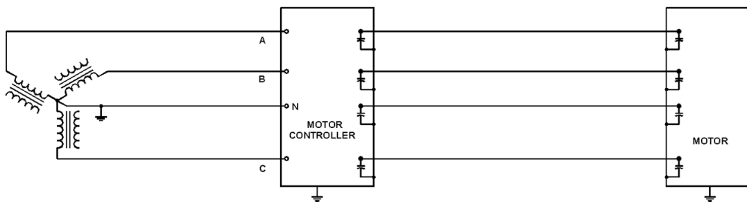
Fig 13 – A Variable Speed Motor and Controller
